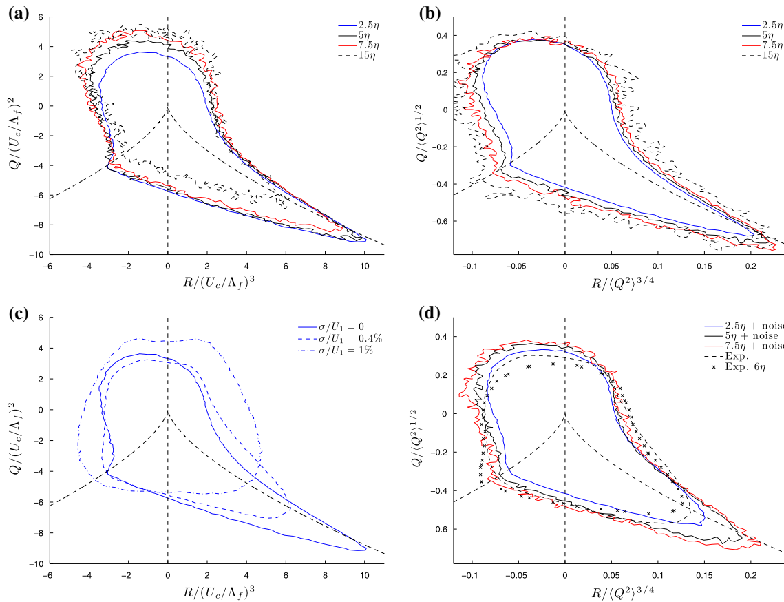
Fig. 11 Joint probability density functions between Q and R a from the numerical datasets normalised by the large-scale quantity, b from the numerical datasets normalised by the local r.m.s. value of Q ( \sqrt{\langle Q^2 \rangle} ) and (d) from the experimental datasets and the numerical datasets to which Gaussian noise has been added, normalised by \sqrt{\langle Q^2 \rangle} . (c) shows the effect of adding Gaussian noise of different
