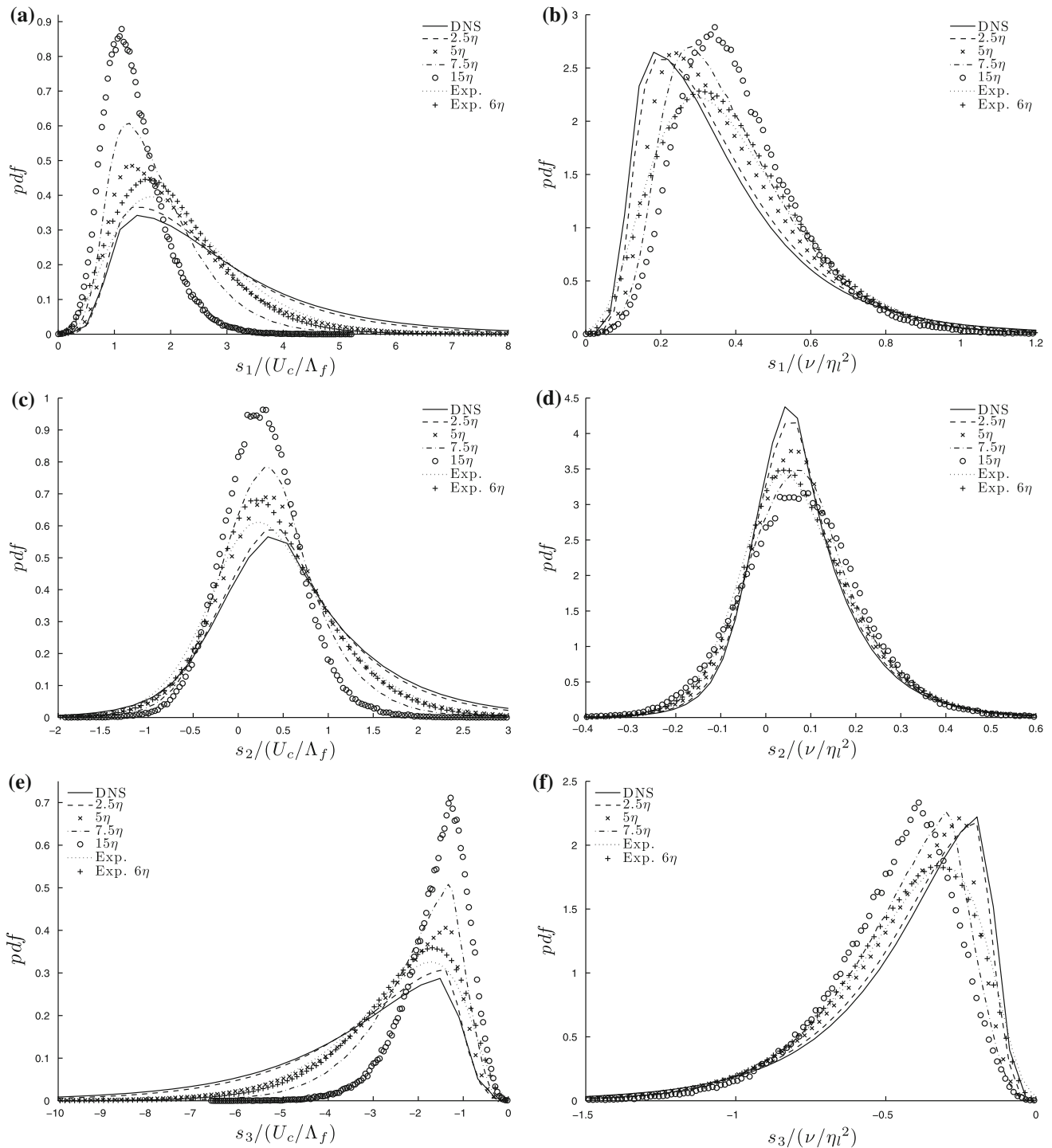
Fig. 8 pdfs of eigenvalues of strain-rate tensor, s_i , normalised by large-scale quantities (left) and the local Kolmogorov length scale (right). Further explanation in the text
