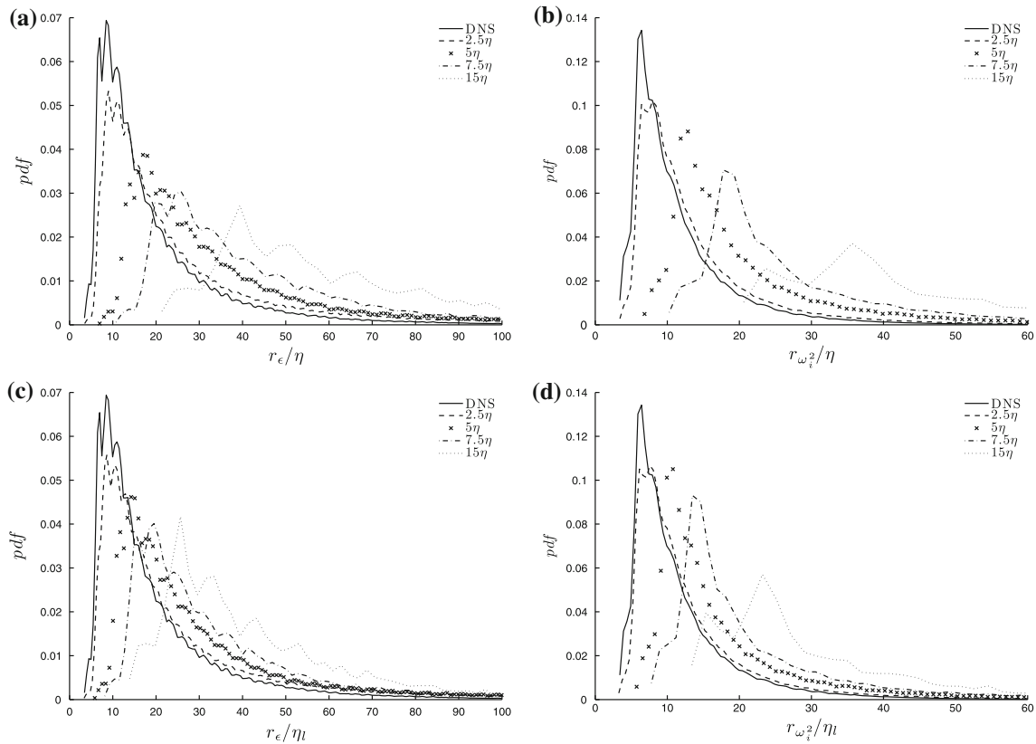
Fig. 5 (a) Probability density function of “diameter” of high dissipation events in the streamwise ( x_1 ) direction in terms of the Kolmogorov length scale calculated from the reference case DNS ( \eta ). (b) pdf of “diameter” of high enstrophy events in the streamwise direction in terms of \eta . (c) pdf of “diameter” of high dissipation
