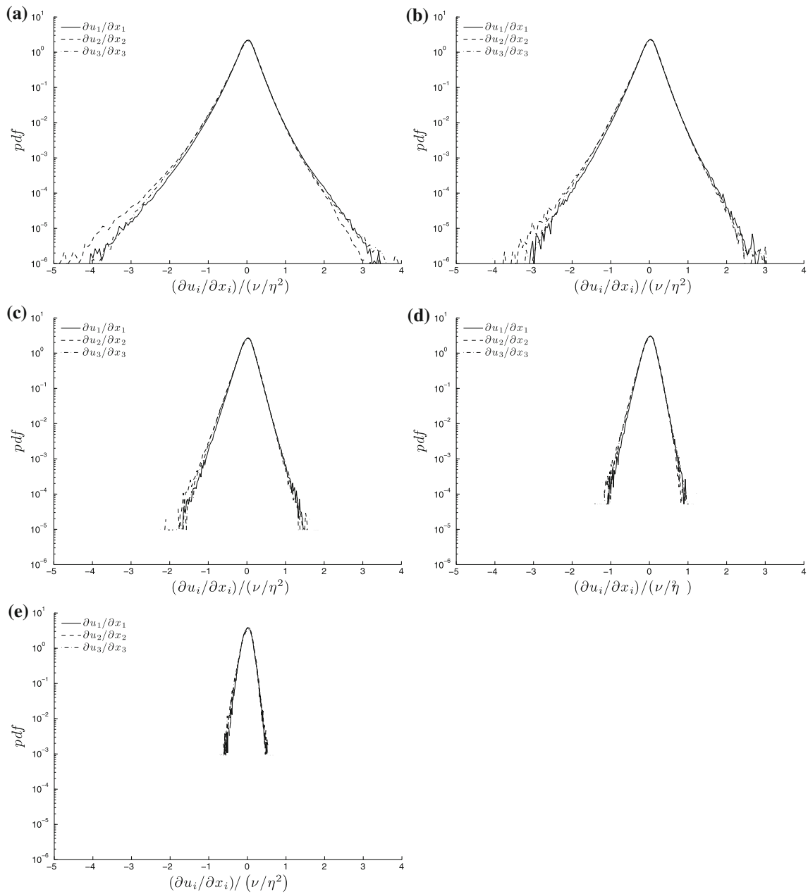
Fig. 1 Probability density functions for the normalised diagonal components of the velocity gradient tensor for (a) the reference DNS dataset, (b) the dataset mean filtered at 2.5\eta , (c) the dataset mean filtered at 5\eta , (d) the dataset mean filtered at 7.5\eta and (e) the dataset mean filtered at 15\eta
