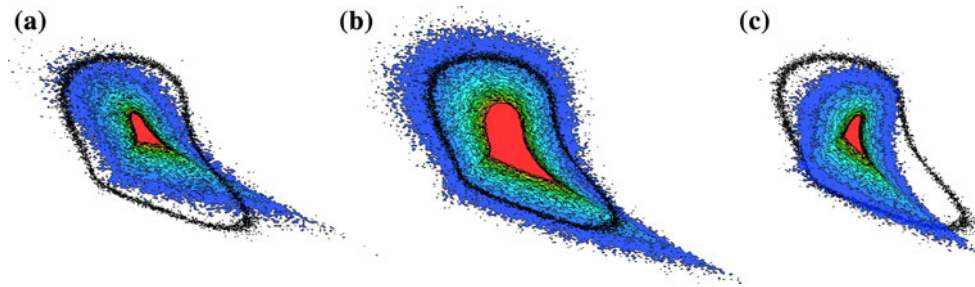
Fig. 12 (a) Slice located at P/(v/\eta^2) = -0.25 illustrating contours of the three-dimensional joint probability density function between P , Q and R from the experimental dataset. (b) Slice located at P/(v/\eta^2) = 0 for the three-dimensional joint pdf . The contour in black
