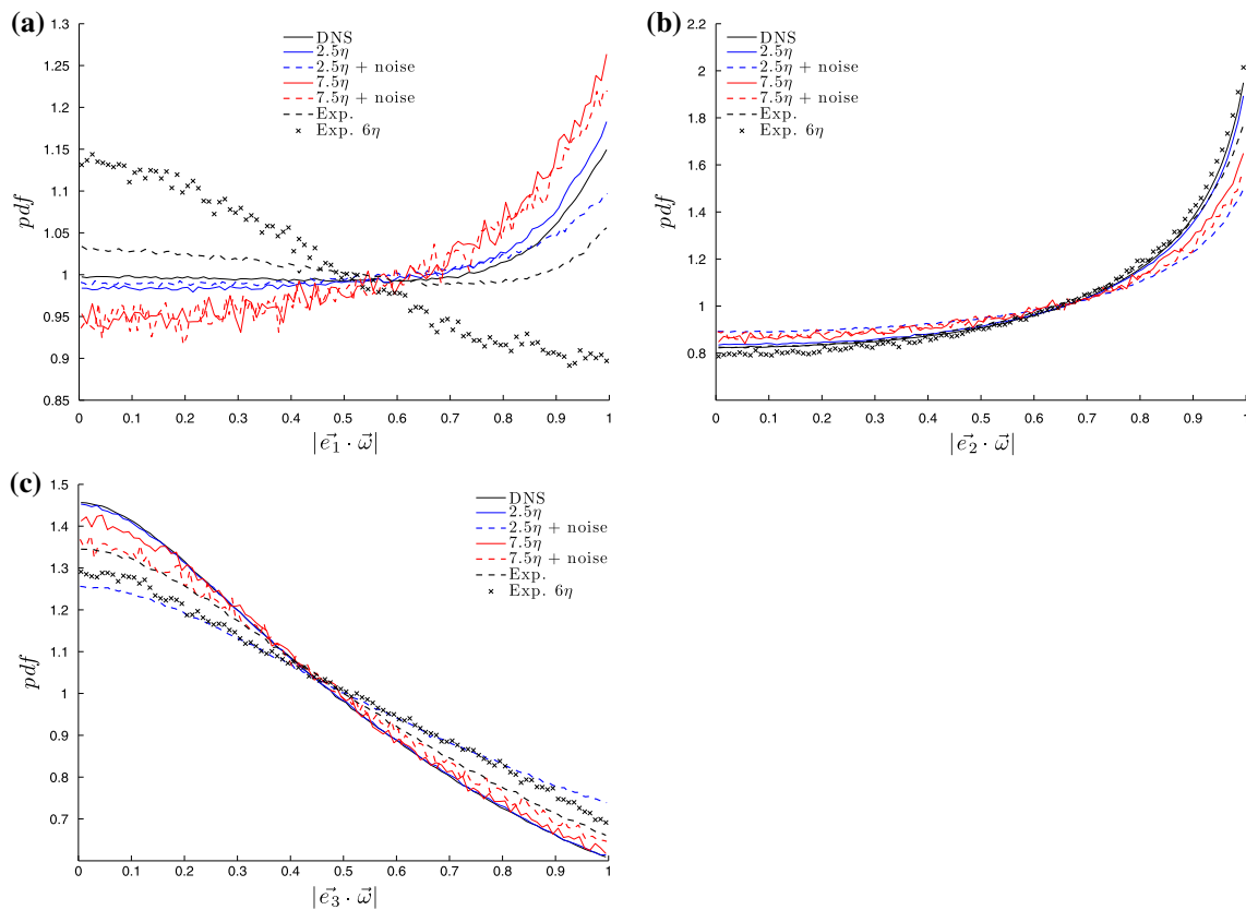
Fig. 14 pdfs of magnitude of alignment cosine between the eigenframe of the strain-rate tensor (a) extensive eigenvector, (b) intermediate eigenvector and (c) compressive eigenvector and the
