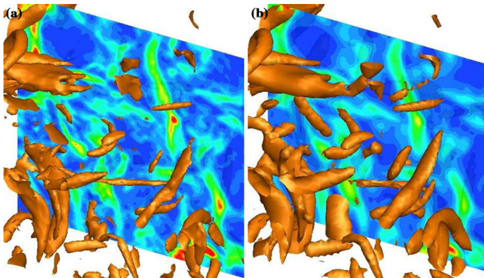
Fig. 7 Isosurfaces of enstrophy ( \omega_i^2 ), where \omega_i^2 is 1% of the global maximum for a the original experimental data, b the experimental data mean filtered at 6\eta . Exactly the same region of the flow is illustrated from exactly the same three-dimensional perspective in
