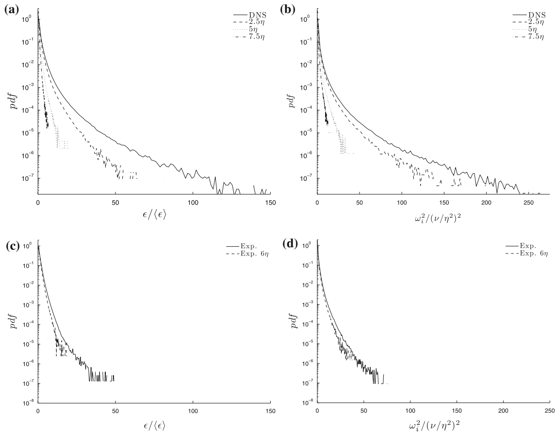
Fig. 3 a Probability density function of dissipation normalised by the mean dissipation rate from the reference case, \langle \epsilon \rangle from the numerical data. b pdf of normalised enstrophy from the numerical data. c pdf of
