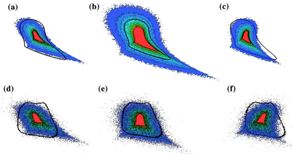
Fig. 13 Slices located at P/(v\eta_1^2) = -0.15 (a), P/(v\eta_1^2) = 0 (b) and P/(v\eta_1^2) = 0.15 (c) for the three-dimensional joint pdf between P , Q and R for the numerical dataset mean filtered at 2.5\eta to which Gaussian noise of variance \sigma/U_1 = 0.4\% has been added. (d), (e) and (f) show slices located at P/(v\eta_1^2) = -0.15 , P/(v\eta_1^2) = 0 and P/(v\eta_1^2) = 0.15 respectively for the P - Q - R 3D joint pdf for the numerical dataset mean filtered at 2.5\eta to which Gaussian noise of variance \sigma/U_1 = 1\% has been added. The contour in black represents the joint pdfs between Q and R from Fig. 11c for the two different noise levels
