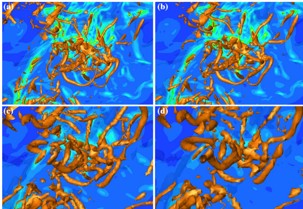
Fig. 6 Isosurfaces of enstrophy ( \omega_i^2 ), where \omega_i^2 is 1% of the global maximum for a the reference DNS case, b the dataset mean filtered at 2.5\eta , c the dataset mean filtered at 5\eta and d the dataset mean filtered at 7.5\eta . Exactly the same region of the flow is illustrated from exactly
