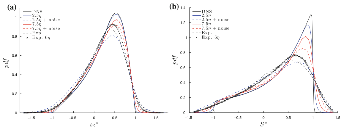
Fig. 10 a pdf for s_2^* (defined in the text) from the numerical data, experimental data and numerical data to which Gaussian noise has been added. b pdf for S^* (defined in the text) from the numerical data, experimental data and numerical data to which Gaussian noise has been added
