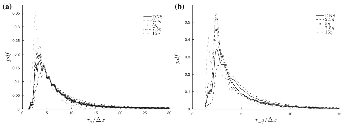
Fig. 4 a Probability density function of “diameter” of high dissipation events in the streamwise ( x_1 ) direction in terms of grid points ( \Delta x ). b pdf of “diameter” of high enstrophy events in the streamwise direction in terms of \Delta x
