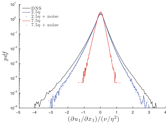
Fig. 9 pdf for the \partial u_1/\partial x_1 component of the velocity gradient tensor normalised by the Kolmogorov length scale from the reference case DNS (c.f. Fig. 1) for the reference case DNS and two of the numerical datasets, both with and without Gaussian noise added
