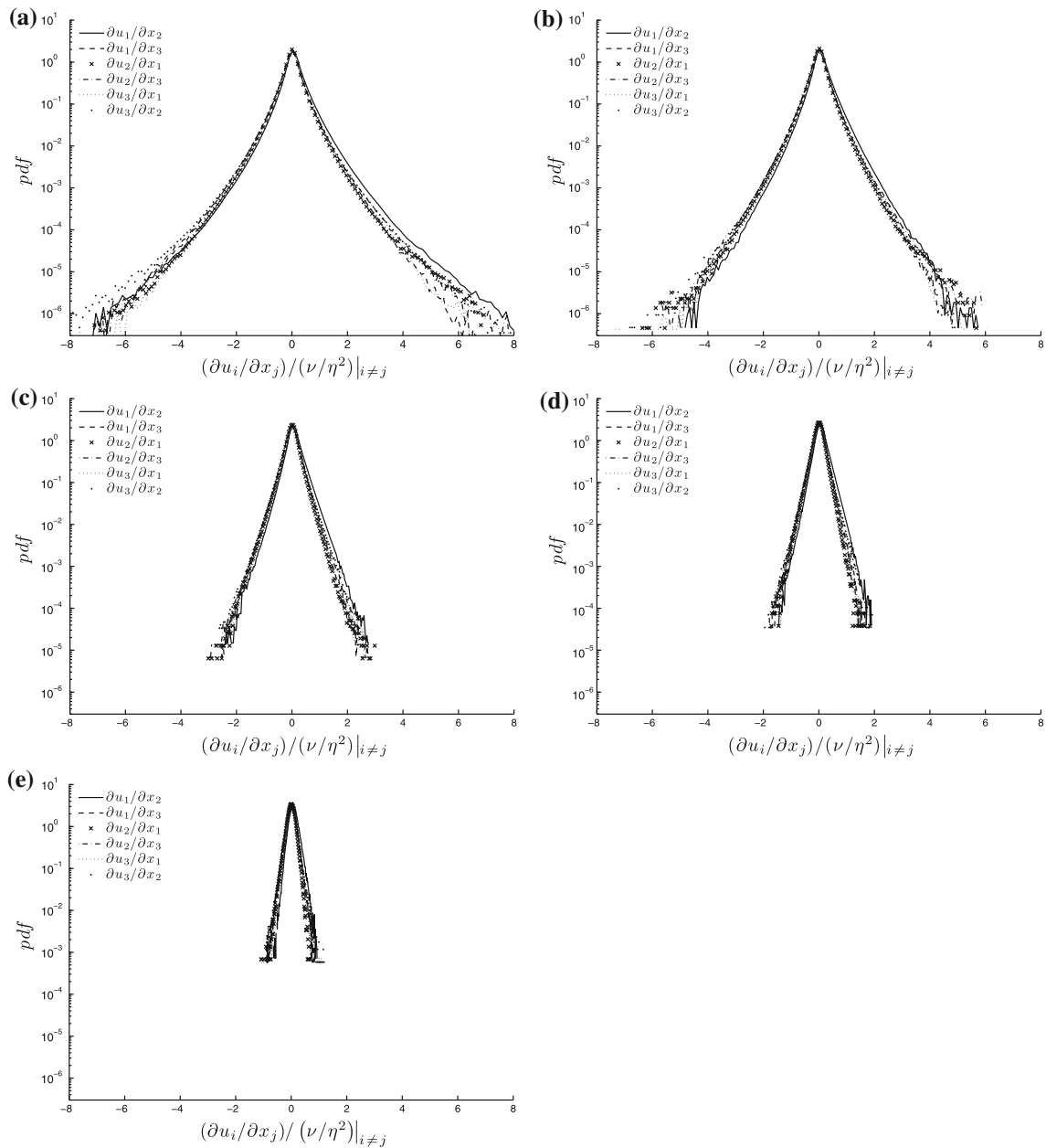
Fig. 2 Probability density functions for the normalised non-diagonal components of the velocity gradient tensor for (a) the reference DNS dataset, (b) the dataset mean filtered at 2.5\eta , (c) the dataset mean
