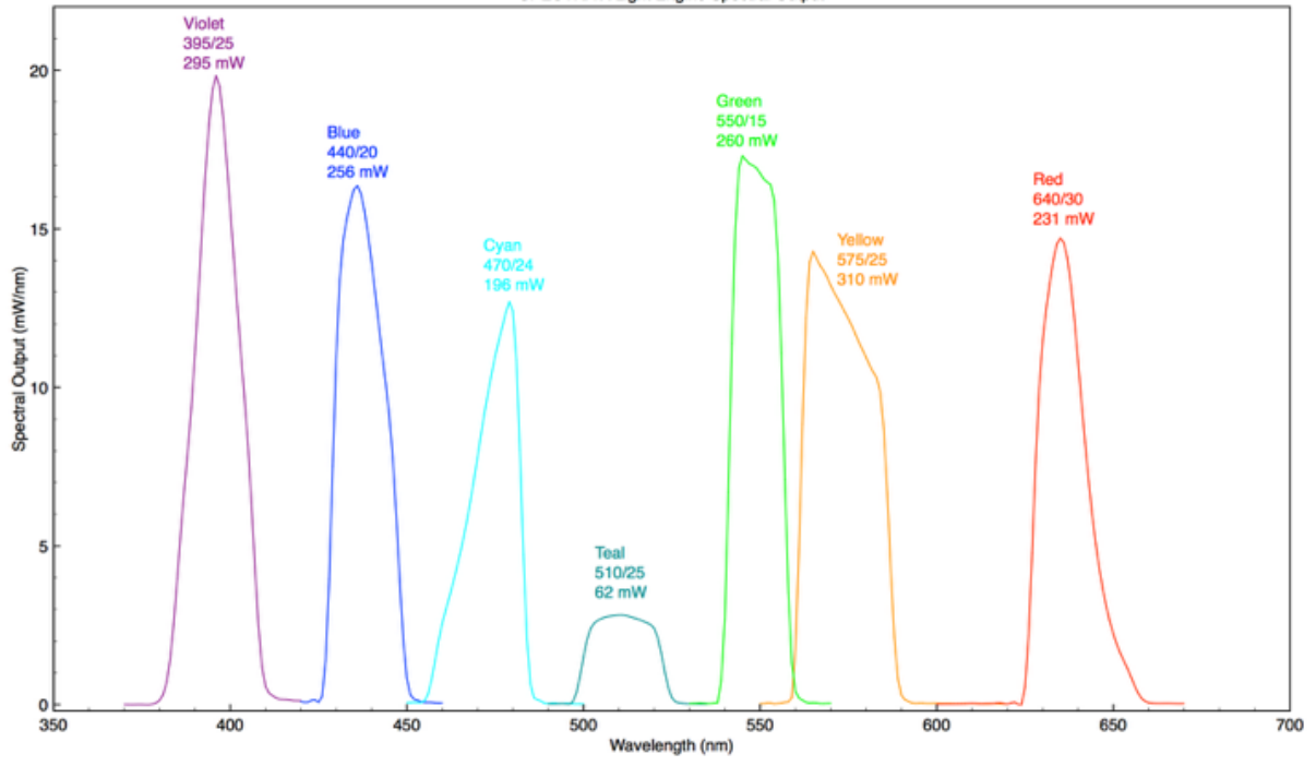
SPECTRA X Light Engine Spectral Output
